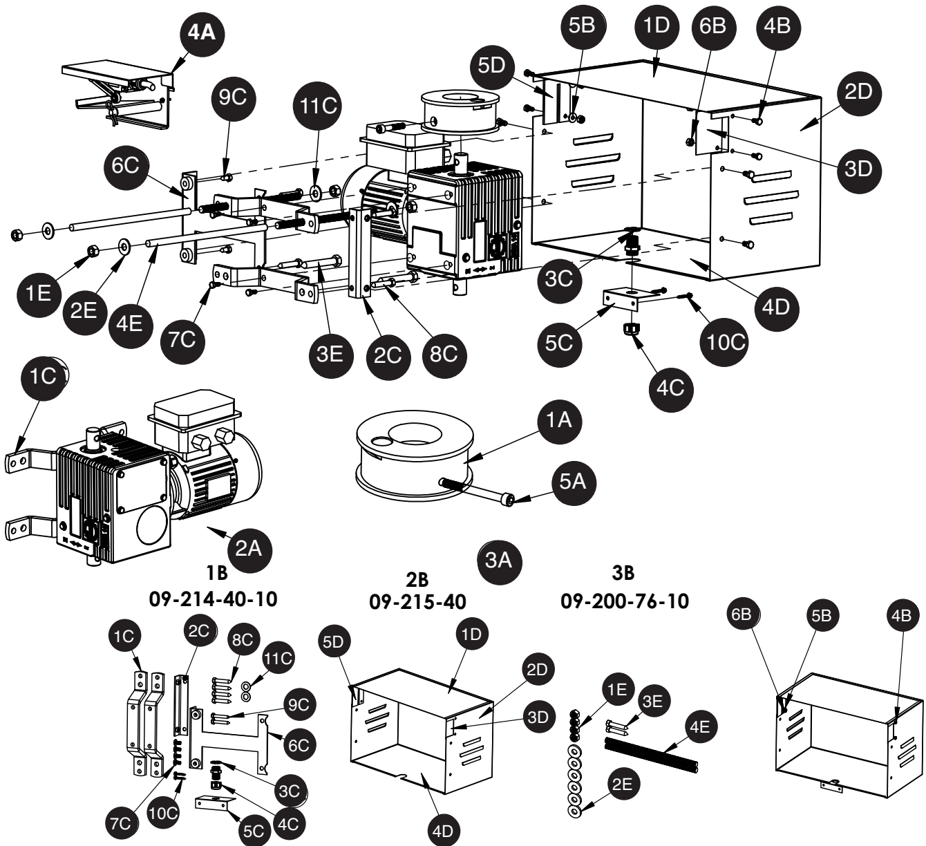
09-314-40 LD DRUM WINCH COVER AND BRACKETS
